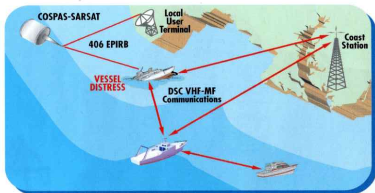
GMDSS BASIC CONCEPT
